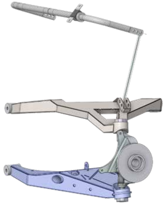
Preparing off-road suspension assembly in Ansys SpaceClaim for simulations
