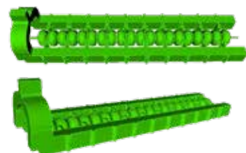
Simulation of linear accelerator designs in Ansys HFSS
