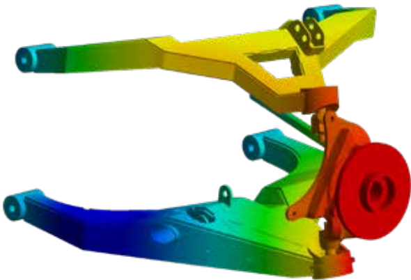
Off-road suspension: simulated displacement field result
