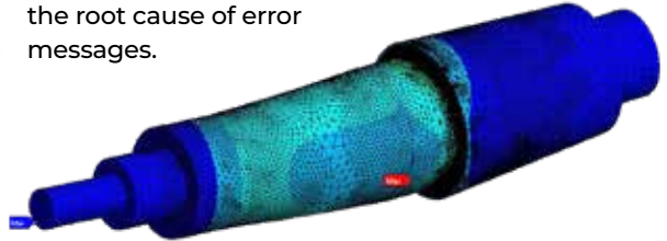
Ansys Mechanical simulation showing maximum stress generated in an axle
