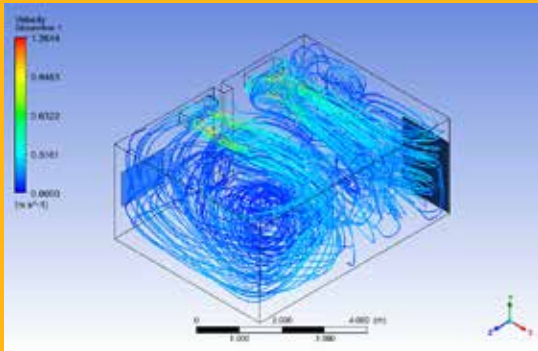
Streamlines depicting the flow path taken by the air entering the room from the air conditioners
