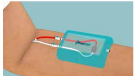
Representation of the CTC-Pheresis concept
