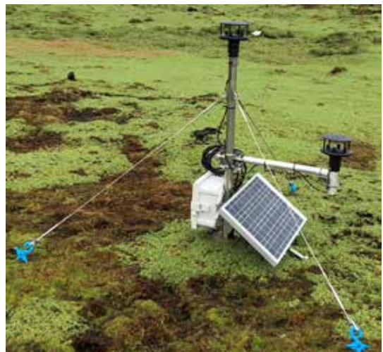
One of 17 wind data logging stations on Marion Island
