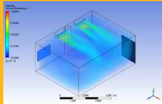
Volume rendering of the velocity of the flow field inside the room
