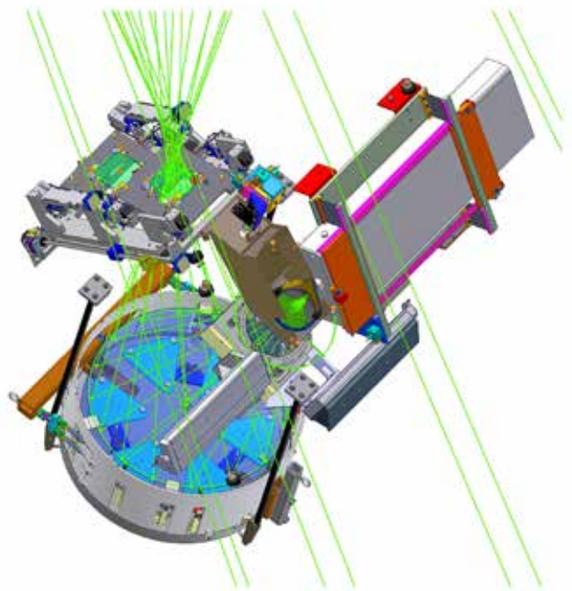
Computer-generated hologram (CGH)-based interferometry configuration for the 8.4-m diameter Giant Magellan Telescope (GMT) off-axis segment surface shape metrology
