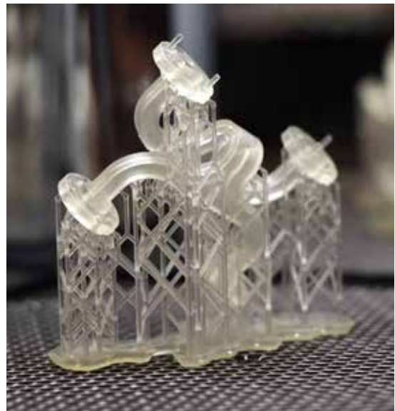
An additively manufactured curvilinear V-band waveguide hybrid coupler designed in HFSS shown before post-processing to remove supports and create conductive walls using pressure-driven electroless metallization
