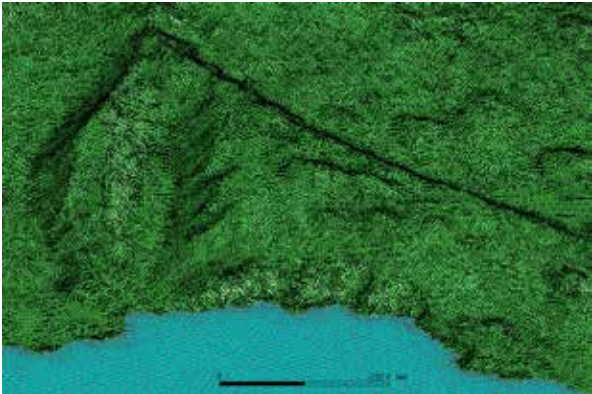
Meshing Marion Island
