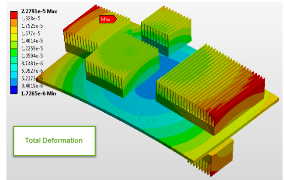
Figure 21. Thermal-induced deformation in Mechanical
