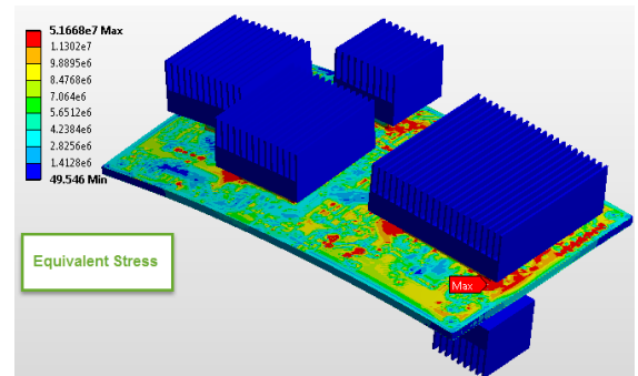
Figure 22. Thermal-induced stress
